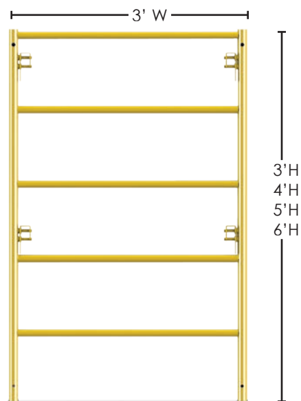
Ladder Frame
